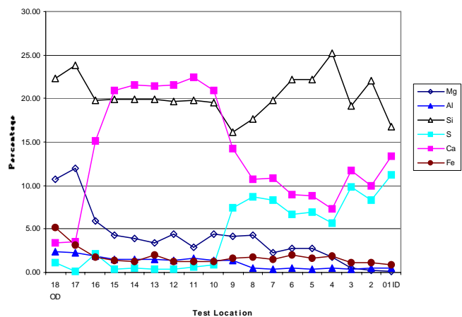
Scanning Electron Microscopy/X-ray Energy Dispersive Spectrography (SEM/EDS) Chemical Analyses Trunk Sewer AC Core Sample No. 2
